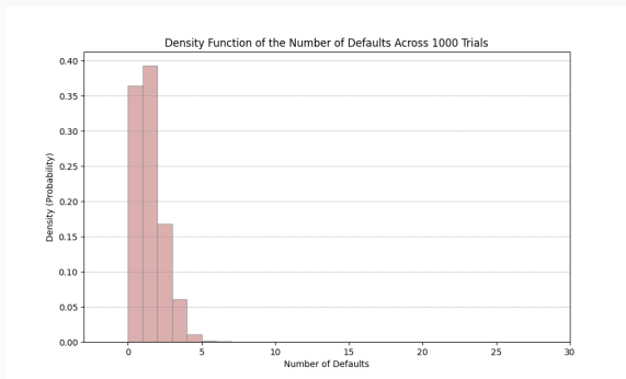
Figure 4: Simulation of Default Outcomes of a Portfolio With No Interdependence: Homogeneous obligors
