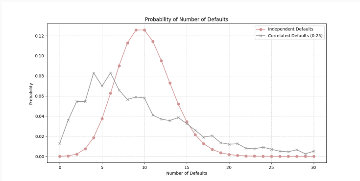
Figure 6: Estimated probability of default numbers
